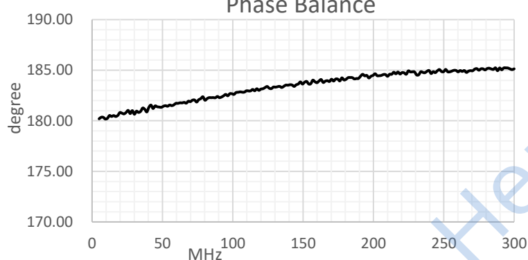
Phase Balance
