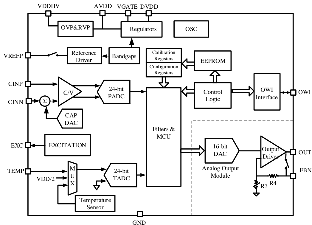
Figure 6.1 Block diagram of the NSC9260
