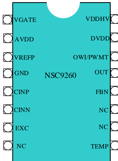
Figure 1.1 NSC9260 Pin Diagram
