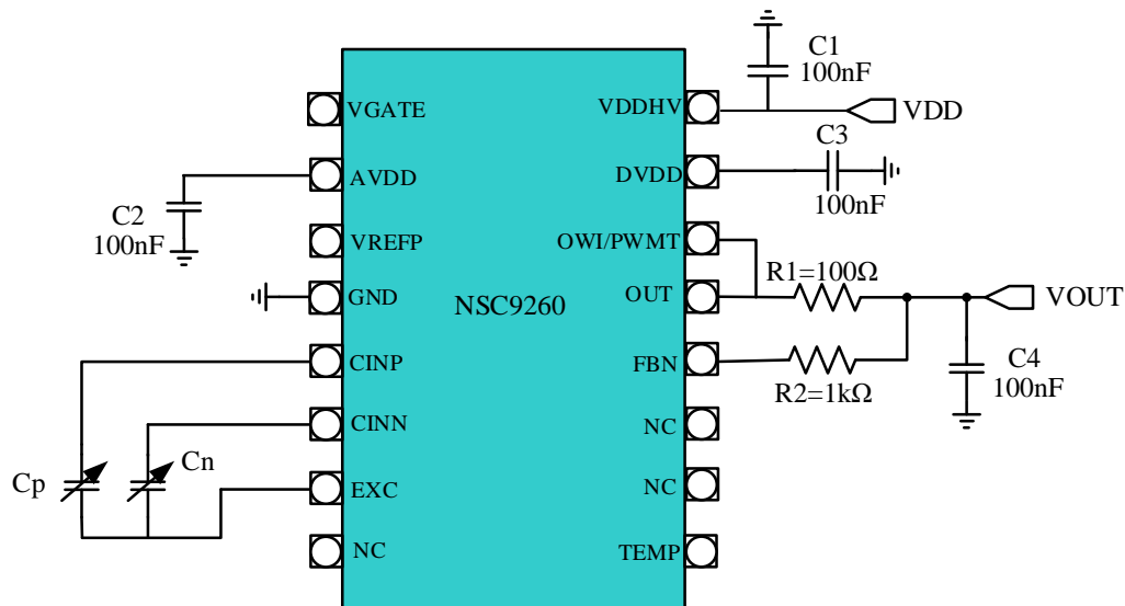
Figure 8.1 Absolute/ratiometric voltage output with Over-voltage Protection
