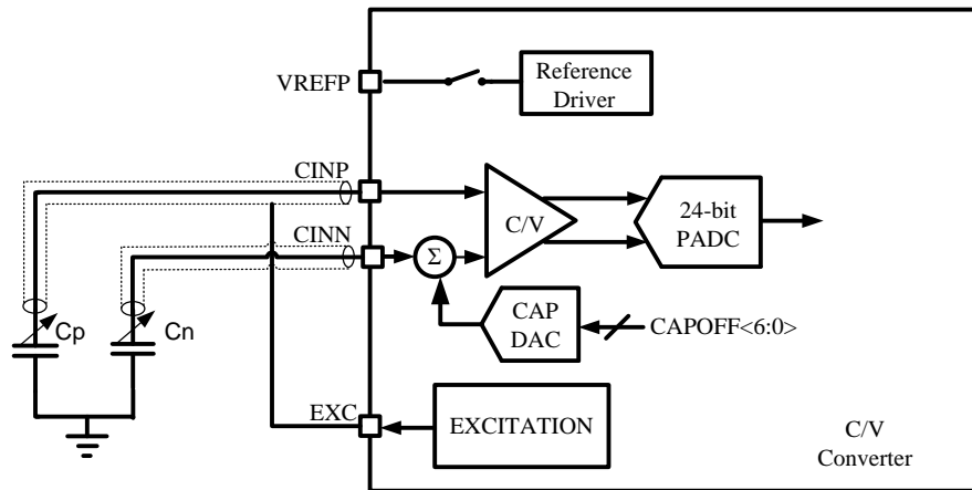
Figure 6.3 C/V converter at Ground Mode (CV_MODE = 1)
