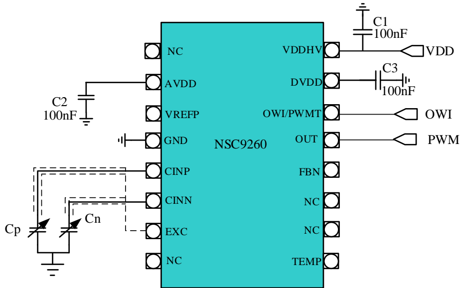
Figure 8.2 Capacitive sensor at Ground Mode with PWM output
