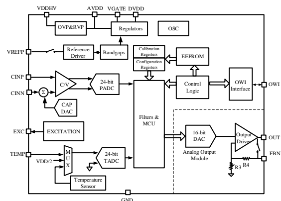
Figure 1. NSC9260 Block Diagram
