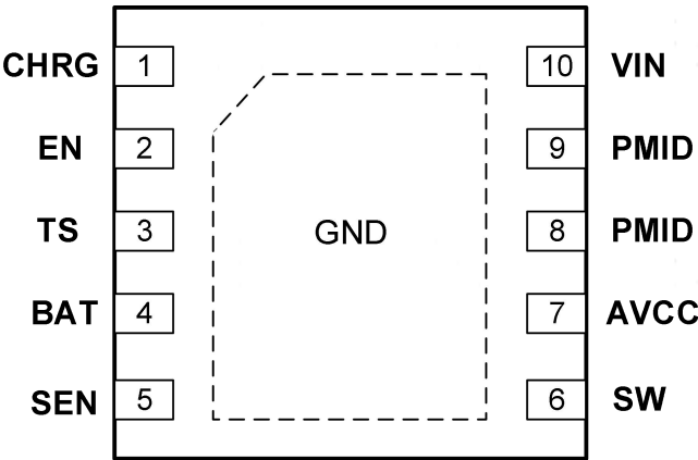
DFN3×3-10L
