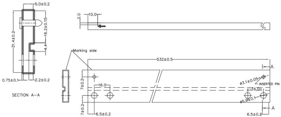
Figure 42. Tube for TO-220 (single gauge) (mm.)
