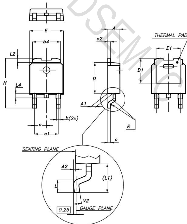
Figure 43. TO-252 package outline
