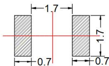
建议焊盘尺寸 Recommended Soldering Pattern
