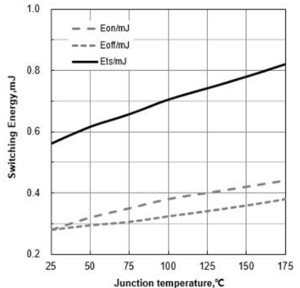
Figure 16. Typical Switching Energy vs Junction Temperature ( V_{CE}=400\text{V} , V_{GE}=15/0\text{V} , I_c=20\text{A} )
