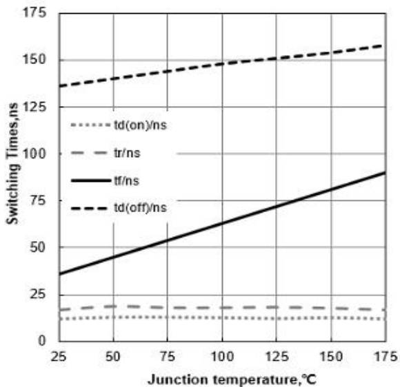
Figure 15. Typical Switching Times vs Junction Temperature ( V_{CE}=400\text{V} , V_{GE}=15/0\text{V} , I_c=20\text{A} )
