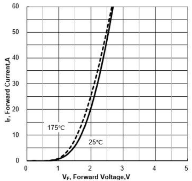
Figure 12. Typical Diode Forward Current vs Forward Voltage
