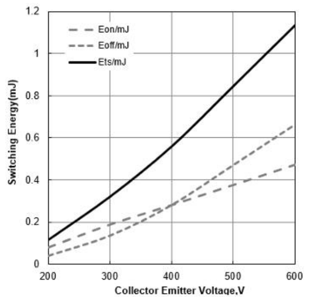
Figure 20. Typical Switching Energy vs V_{CE} ( T_J=25^\circ\text{C} , V_{GE}=15/0\text{V} , I_c=20\text{A} )
