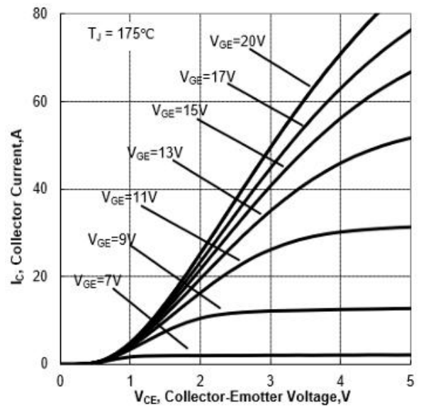
Figure 8. Typical Output Characteristics ( T_J=175^\circ\text{C} )
