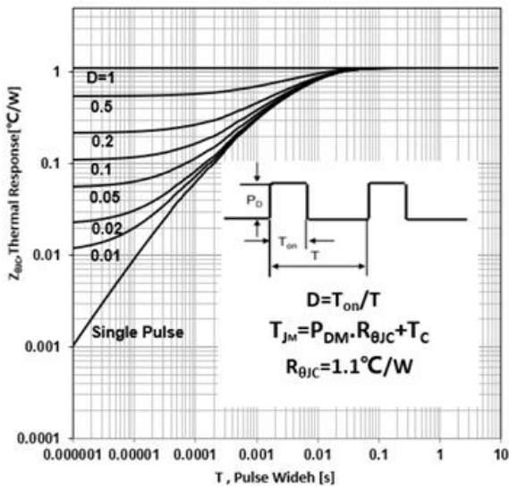
Figure 23. IGBT Transient Thermal Impedance vs Pulse Width(TO220)
