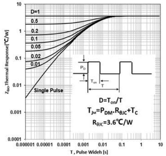
Figure 26. Diode Transient Thermal Impedance vs Pulse Width(TO220F)
