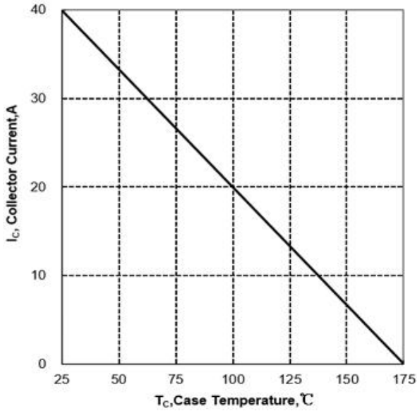
Figure 5. Collector Current vs Case Temperature for TO220
