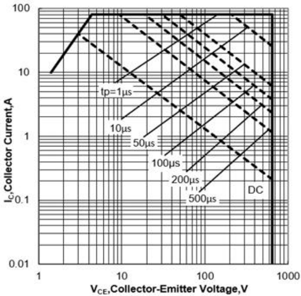
Figure 1. Forward Bias Safe Operating Area for TO220
