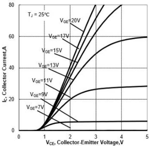
Figure 7. Typical Output Characteristics ( T_J=25^\circ\text{C} )
