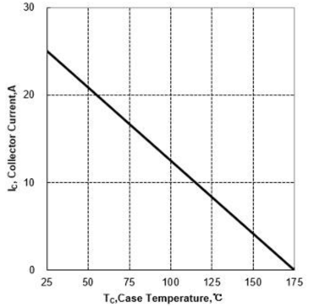
Figure 6. Collector Current vs Case Temperature for TO220F
