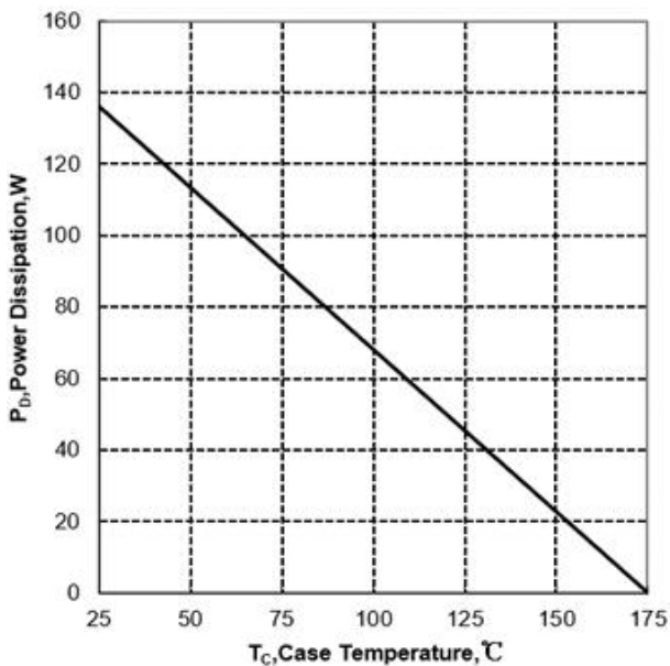
Figure 3. Power Dissipation vs Case Temperature for TO220
