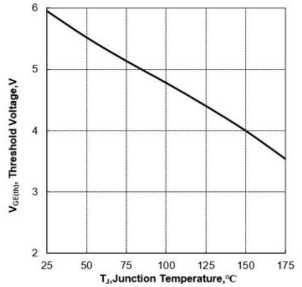
Figure 10. Typical Gate-Emitter Threshold Voltage vs Junction Temperature
