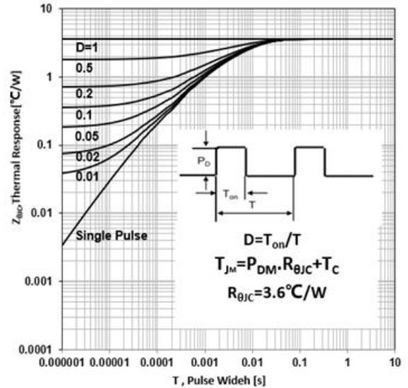
Figure 24. IGBT Transient Thermal Impedance vs Pulse Width(TO220F)
