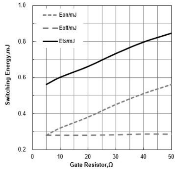
Figure 14. Typical Switching Energy vs Gate Resistor ( T_J=25^\circ\text{C} , V_{CE}=400\text{V} , V_{GE}=15/0\text{V} , I_c=20\text{A} )
