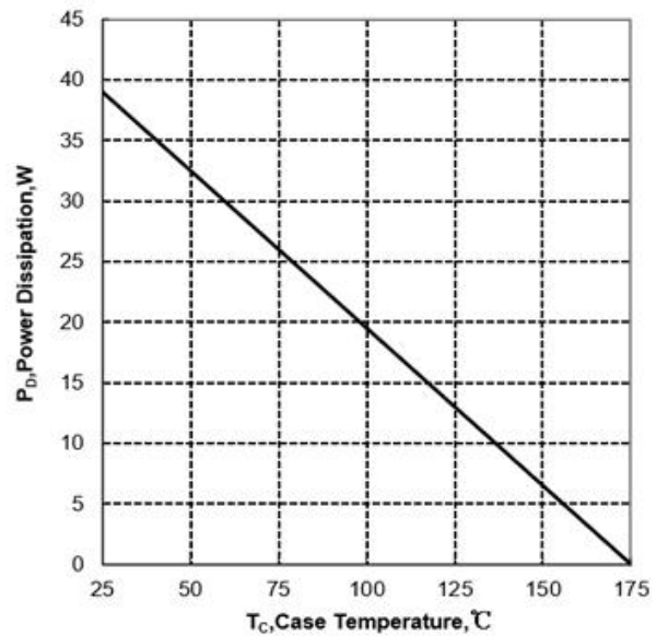
Figure 4. Power Dissipation vs Case Temperature for TO220F
