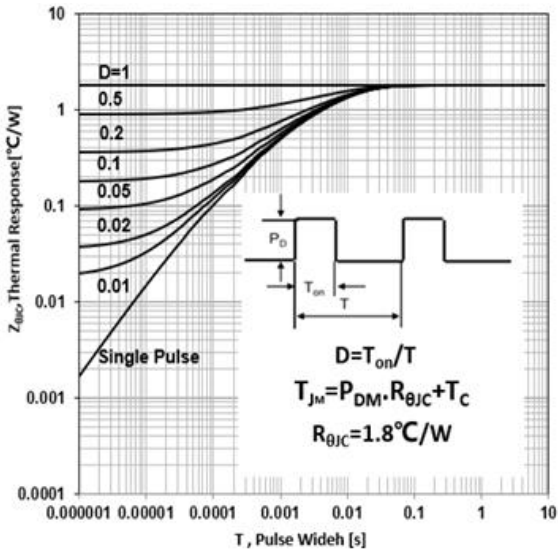
Figure 25. Diode Transient Thermal Impedance vs Pulse Width(TO220)
