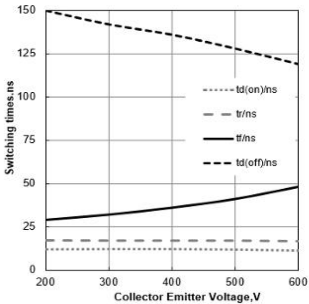
Figure 19. Typical Switching Times vs V_{CE} ( T_J=25^\circ\text{C} , V_{GE}=15/0\text{V} , I_c=20\text{A} )
