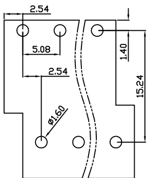
PCB Layout
