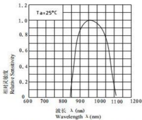
Fig.4 Relative Sensitivity vs. Wavelength
