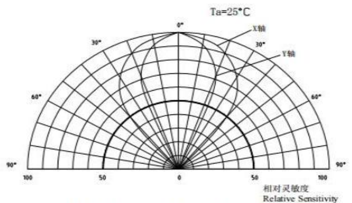
Fig.5 Relative Directional Sensitivity
