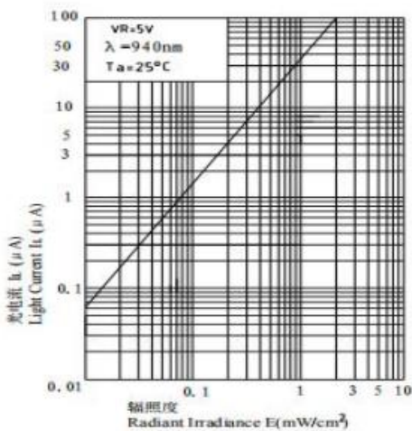
Fig.2 Light Current vs. Irradiance
