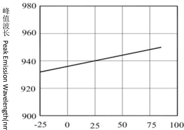
Peak Emission Wavelength vs. Ambient Temperature
