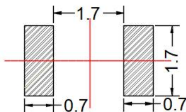
建议焊盘尺寸 Recommended Soldering Pattern
