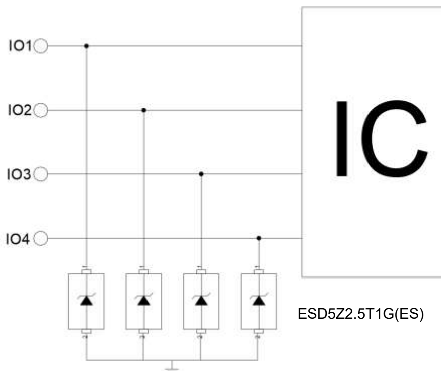
Pic-1 Typical Internet 1G Interface Application
