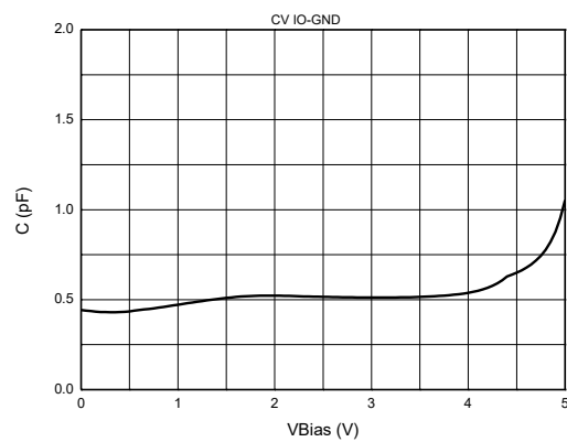
Figure2: Junction Capacitance vs. Reverse Voltage
