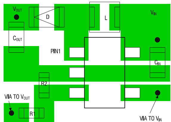
Figure 3. MIC2288YD5-MS Suggested Layout
