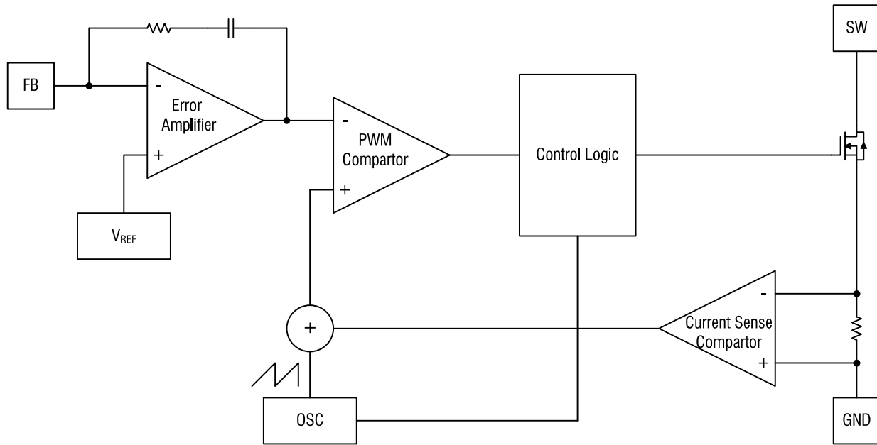
Figure 2. MIC2288YD5-MS Block Diagram
