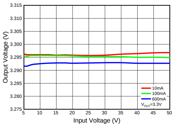
(5) Output Voltage VS Input Voltage ( V_{\text{OUT}}=3.3\text{V} )
