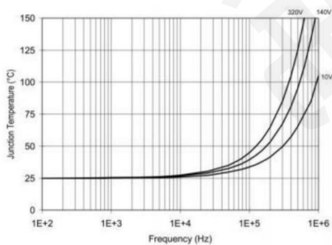
Figure 31. TJ vs. Frequency(IRFPE50) RGATE = 10Ω, VCC = 15V
