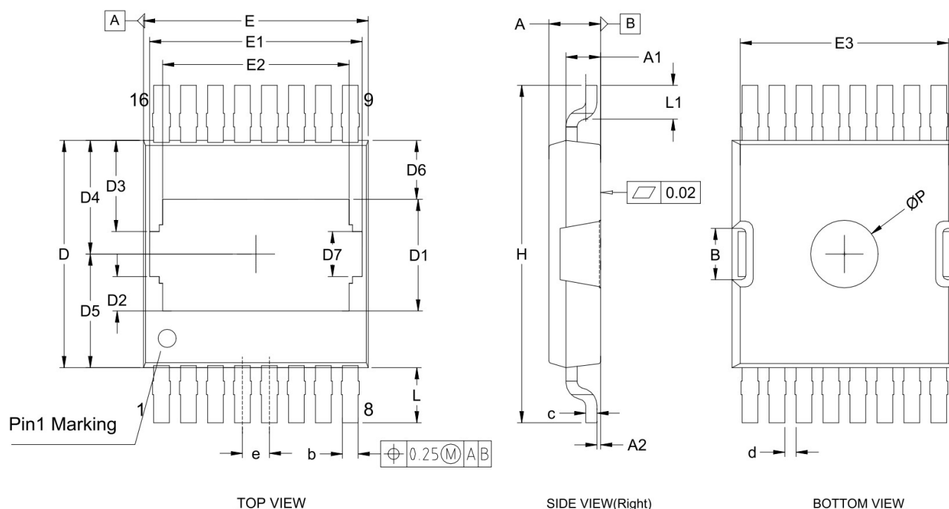
Figure 1. Outline TOLT, dimensions in mm/TOLT外形尺寸 (毫米)
