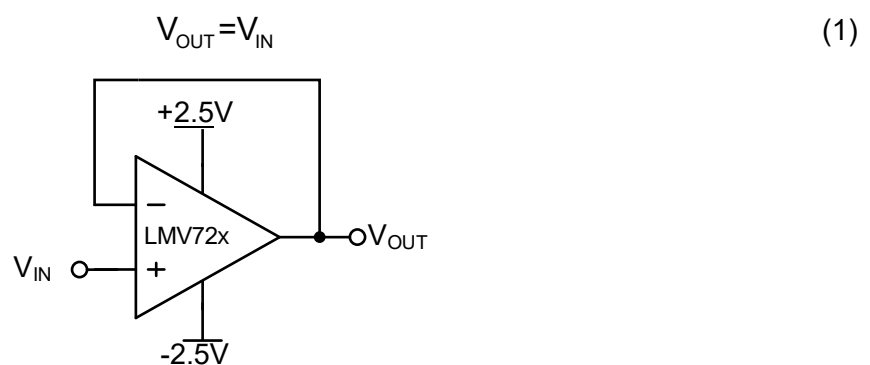
Figure 17. Voltage Follower
