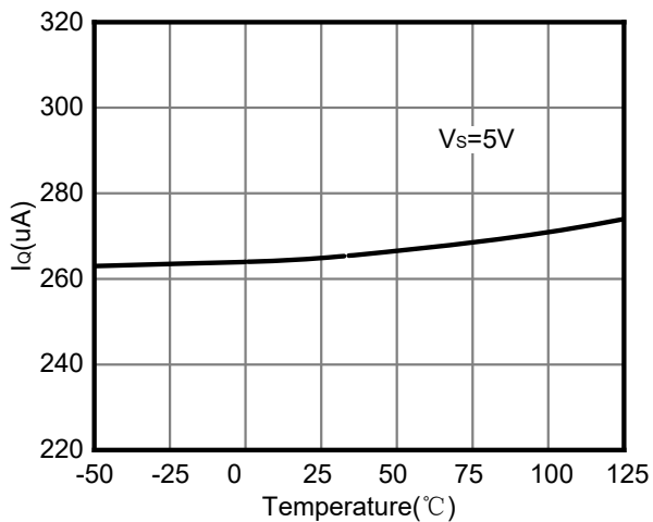
Figure 6. Quiescent Current vs Temperature
