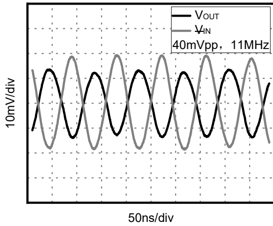
Figure 14. -3dB bandwidth
