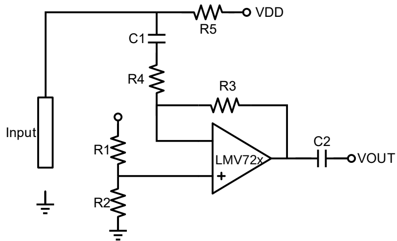
Figure 1. Typical Application
