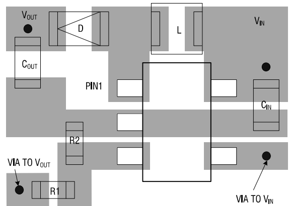
Figure 3. MCP1661T-E/OT-MS Suggested Layout
