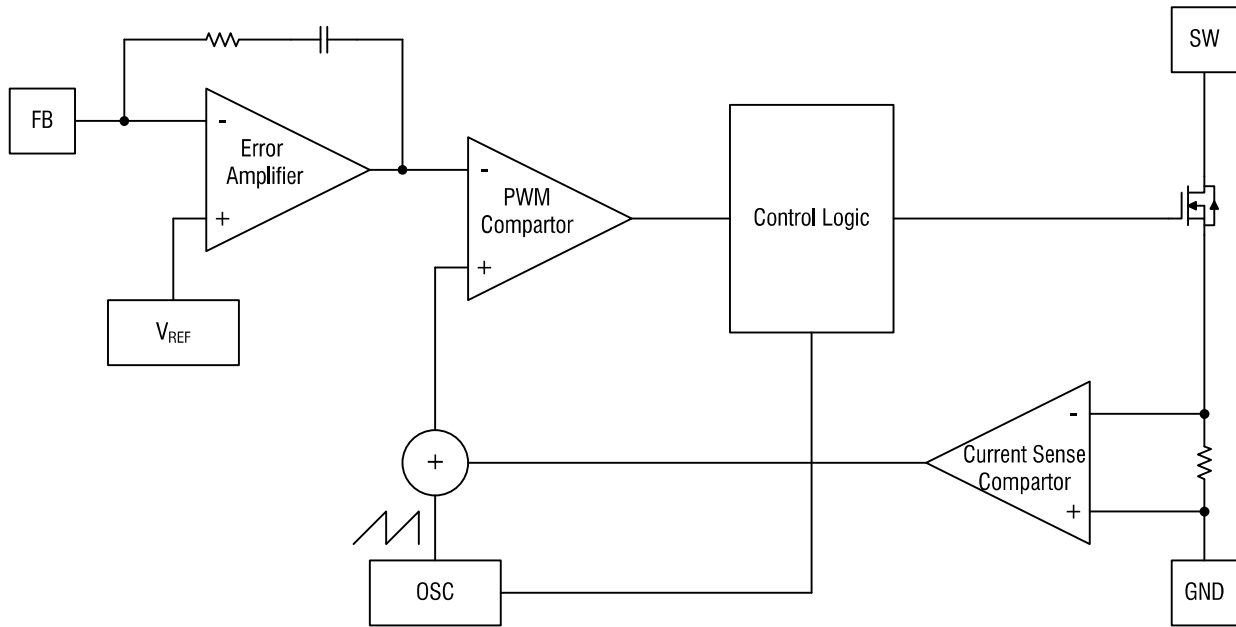
Figure 2. MCP1661T-E/OT-MS Block Diagram
