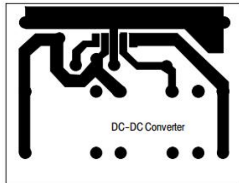
NOTE: Not to scale. Figure 37. Printed Circuit Board Copper Side
