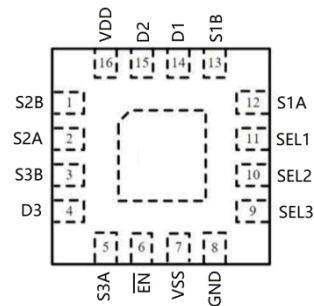
QFN-16
