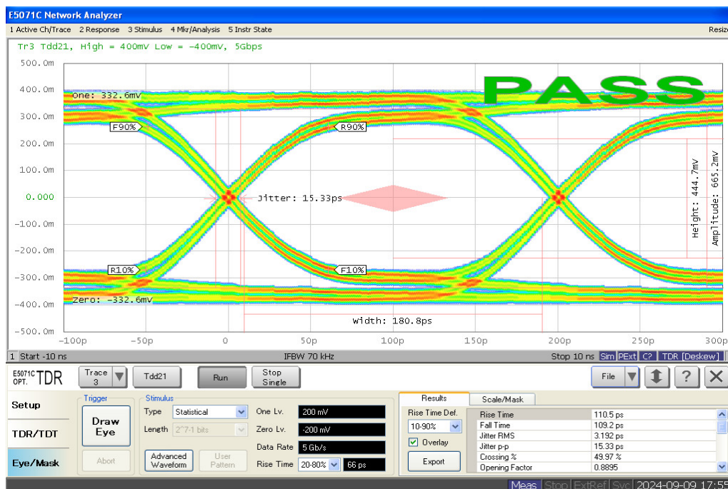
USB3.2 Gen1 Eye Diagram W/I Device (5Gbps)
