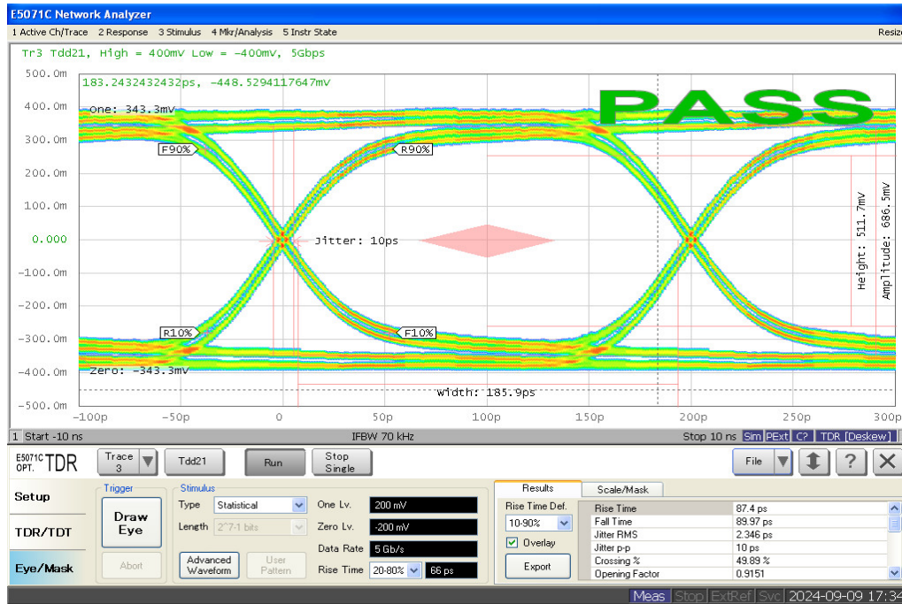
USB3.2 Gen1 Eye Diagram W/O Device (5Gbps)
