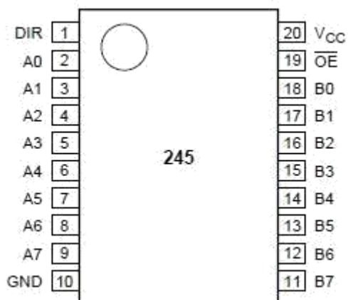
DIP-20/SOP-20W/TSSOP-20
