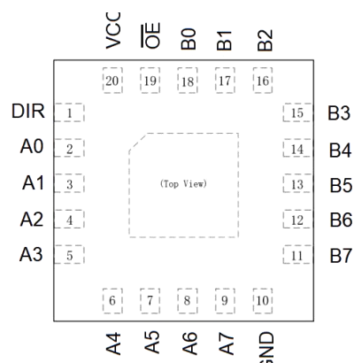
QFN-20 4*4
