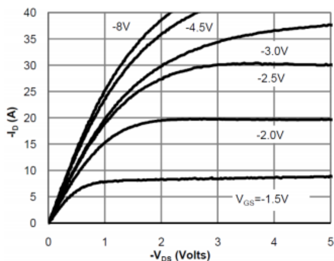
Fig 1: On-Region Characteristics
