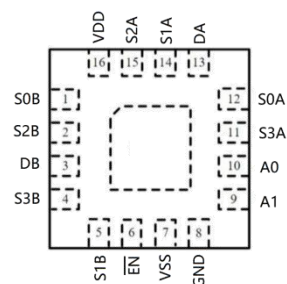
QFN-16
