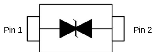
SOD 323 (Top View)
