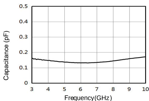
Capacitance vs Frequency of I/O to I/O
