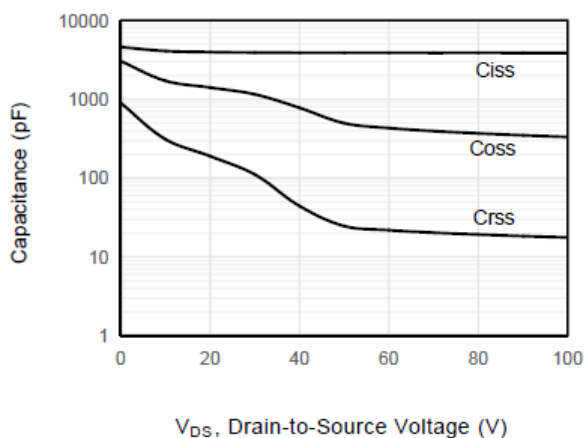
Figure 6 . Capacitance
