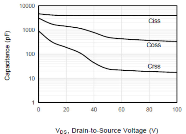
Figure 6 . Capacitance
