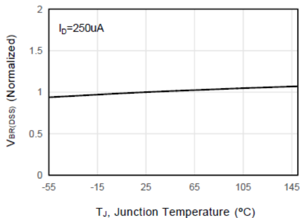
Figure 9. Breakdown Voltage vs Junction Temperature
