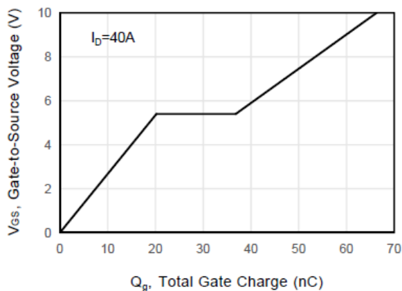
Figure 7 . Gate Charge
