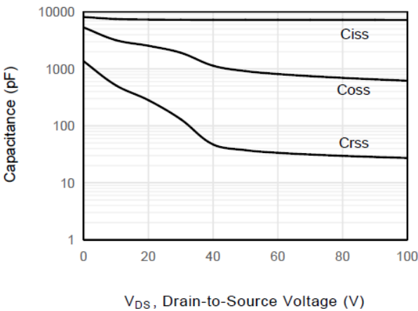
Figure 6 . Capacitance
