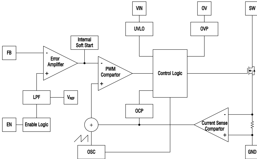
Figure 2. AP3031KTR-MS Block Diagram
