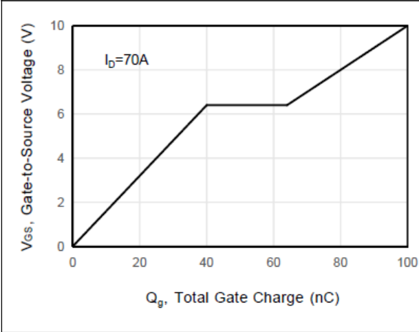
Figure 7 . Gate Charge
