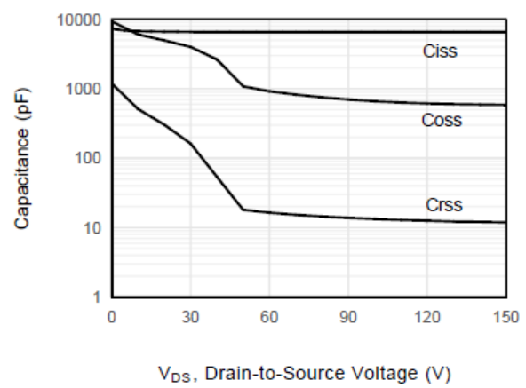
Figure 6 . Capacitance
