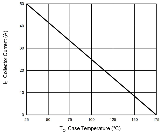
Figure 18 I_C vs. Temperature
