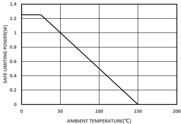
Figure 9. Thermal Derating Curve, Dependence of Safety Limiting Values with Ambient Temperature per VDE (left: ADuM120x; right: ADuM130x)
