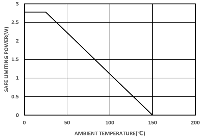
Figure 9. Thermal Derating Curve, Dependence of Safety Limiting Values with Ambient Temperature per VDE (left: ADuM120x; right: ADuM130x)
