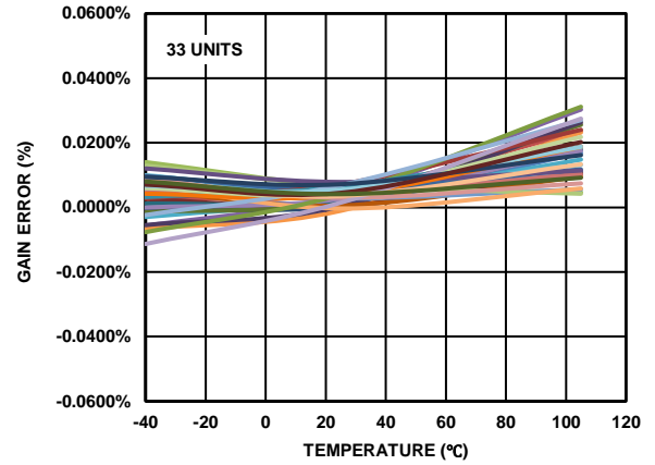
Figure 14: Gain Error G=16, Mid Power Mode
