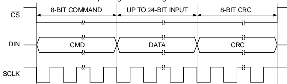
Figure 49: SPI Write Transaction with CRC
