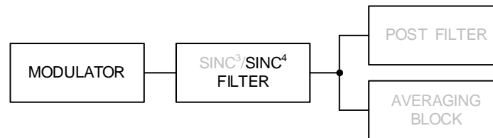
Figure 34: Sinc 4 Filter
