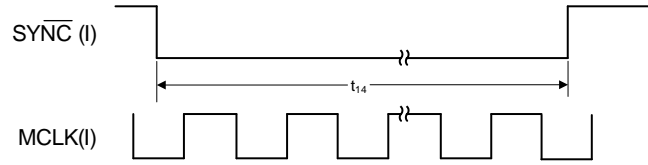
Figure 6: SYNC Pulse Width
