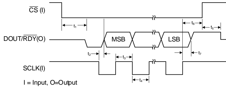
Figure 1: Read Cycle Timing Diagram ( \overline{\text{CS\_EN}} Bit Cleared)
