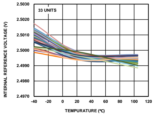
Figure 18: Internal Reference Voltage vs. Temperature
