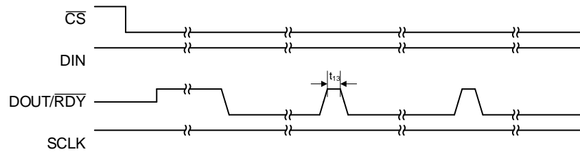
Figure 5: \overline{DOUT}/\overline{RDY} High Time when \overline{DOUT}/\overline{RDY} is Initially Low and the Next Conversion is Available
