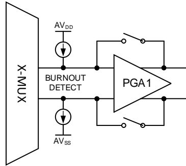
Figure 51: Burnout Currents
