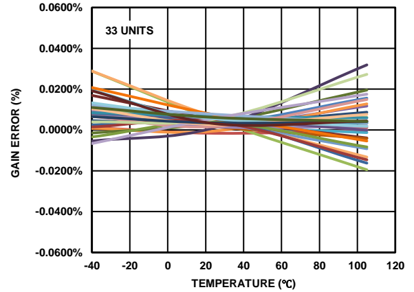
Figure 16: Gain Error G=16, Low Power Mode
