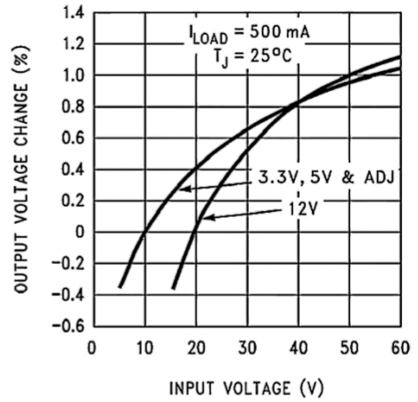
Line Regulation
