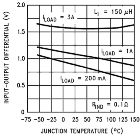
Dropout Voltage
