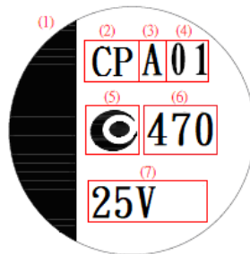
Figure 3 Marking
