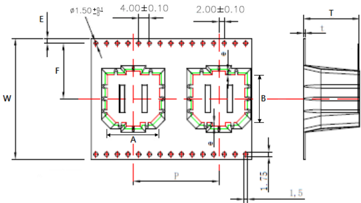
Fig. 6 Carrier tape
