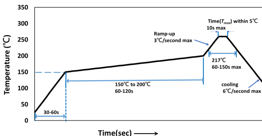
Figure 4 Reflow profile
