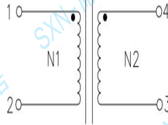
SCHMATIC
