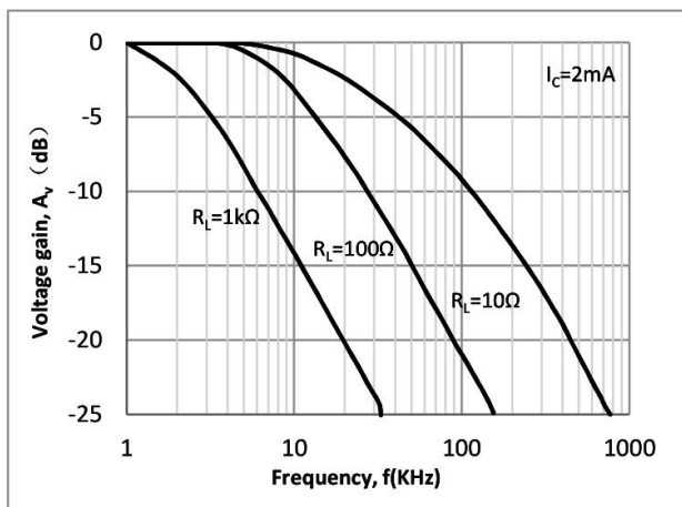
Fig.9 Frequency response
