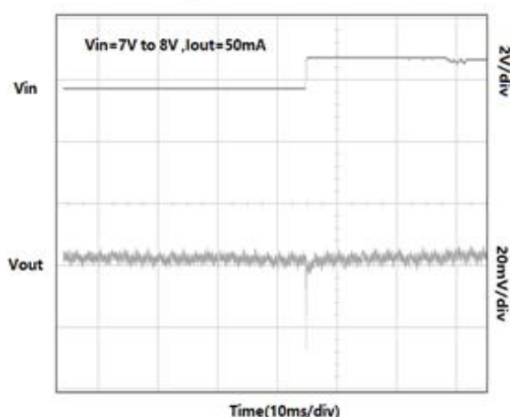
Line-transient Response
