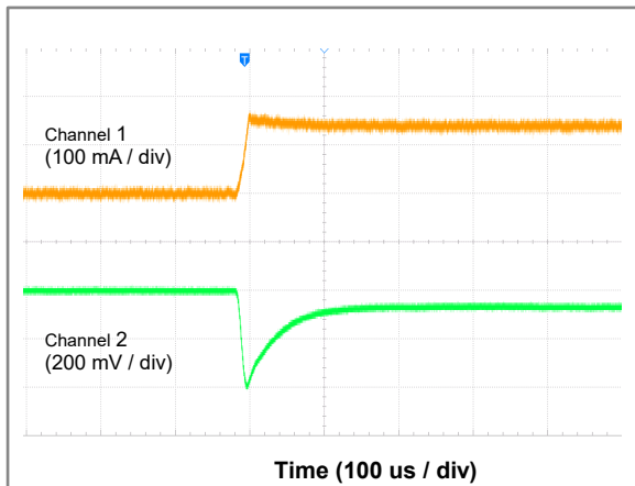
Figure 19. Load Transient (1 mA to 150 mA)
