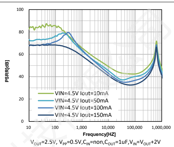
Figure 35. PSRR vs Frequency
