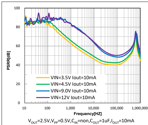
Figure 34. PSRR vs Frequency
