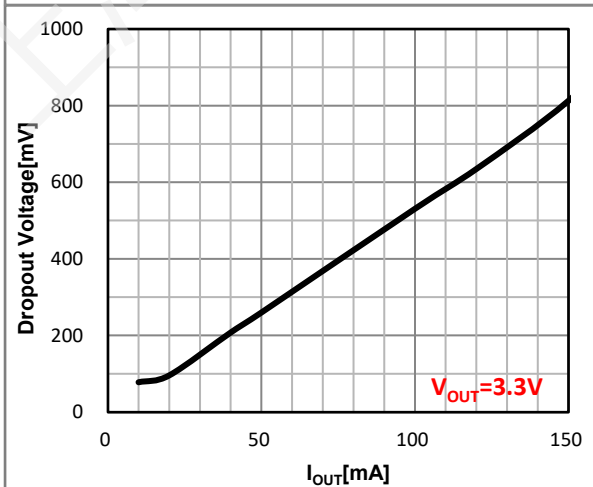
Figure 5. Dropout Voltage VS I_{OUT}
