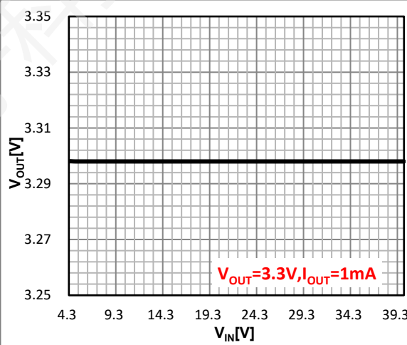
Figure 10. Line Regulation
