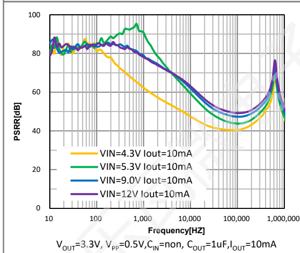
Figure 36. PSRR vs Frequency
