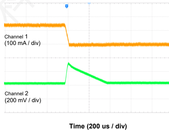
Figure 22. Load Transient (150 mA to 1 mA)
