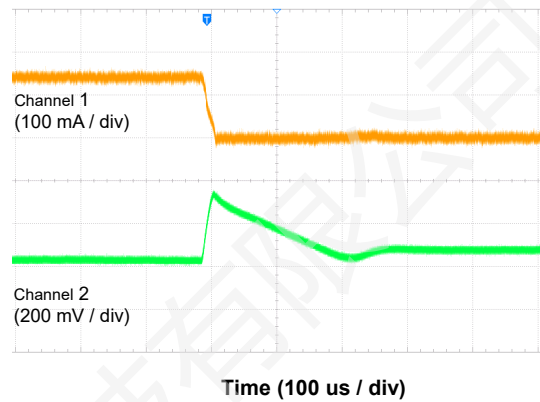
Figure 20. Load Transient (150 mA to 1 mA)
