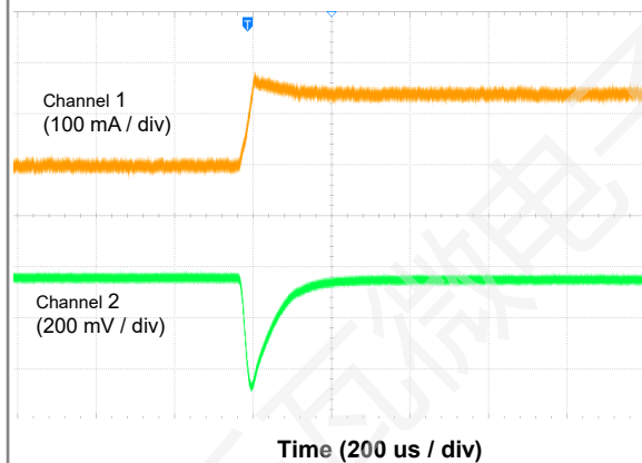
Figure 21. Load Transient (1 mA to 150 mA)
