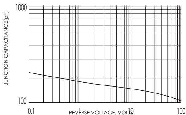
FIG.5-TYPICAL JUNCTION CAPACITANCE
