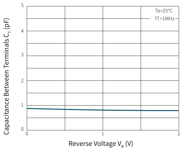
Fig.3 C_j — V_R
