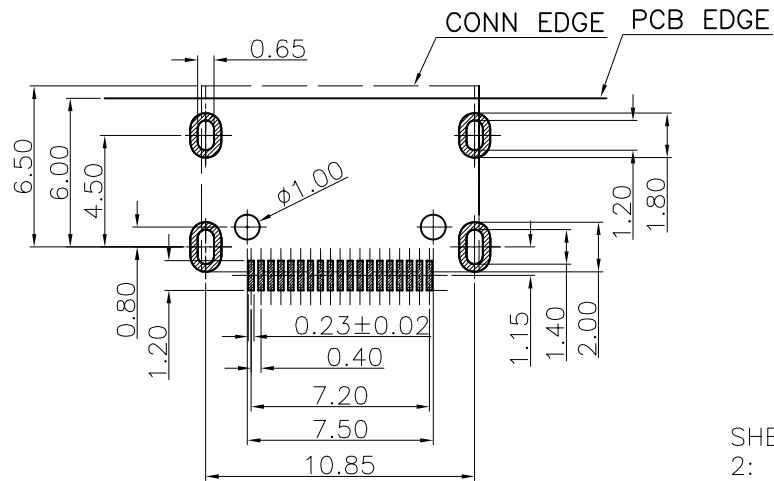
RECOMMENDED PCB LAYOUT(TOP VIEW) (THICKNESS=0.8±0.05mm) TOLERANCE = ±0.05
