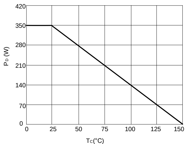
Figure 10: Power De-rating
