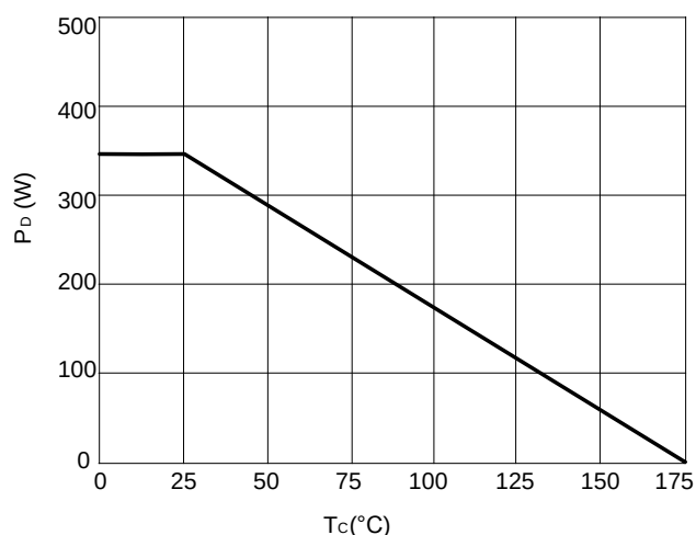
Figure 8: Power De-rating
