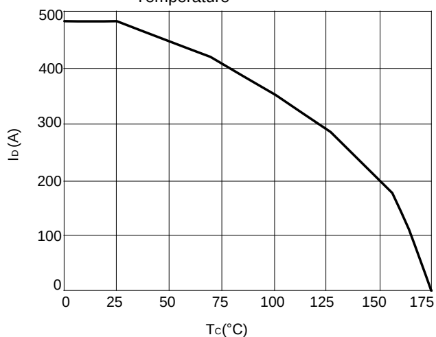
Figure 9: Current De-rating
