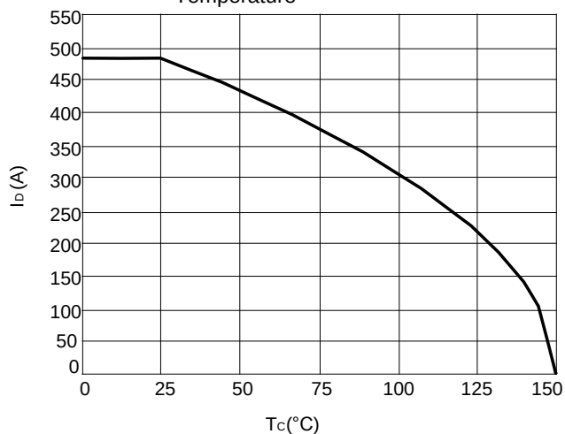
Figure 11: Current De-rating
