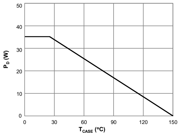
Figure 8: Power De-rating
