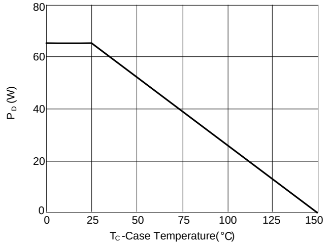
Figure 8: Power De-rating
