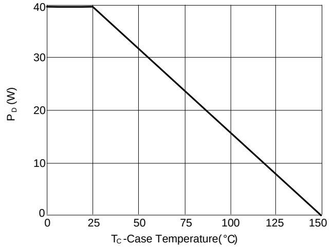
Figure 8: Power De-rating
