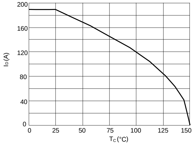
Figure 8: Current De-rating
