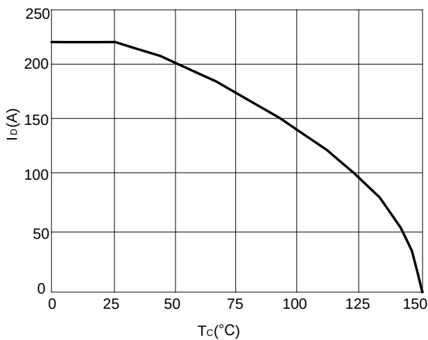
Figure 11: Current De-rating
