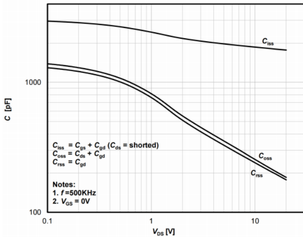
Figure 5. Capacitance Characteristics
