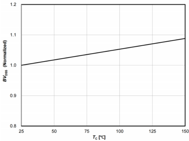
Figure 7. Normalized BV_{DSS} vs. Temperature
